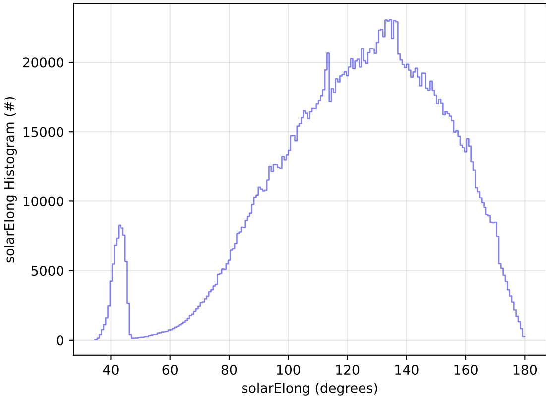
ddf_acor_sf25_lsf40_lsr20_v3.4_10yrs WFD all bands: solarElong Histogram
