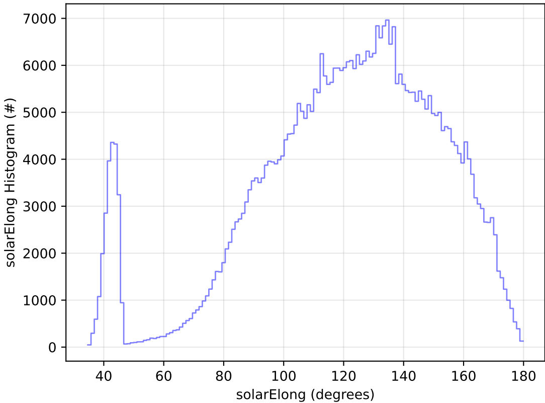
ddf_acor_sf25_lsf40_lsr20_v3.4_10yrs All sky z band: solarElong Histogram
