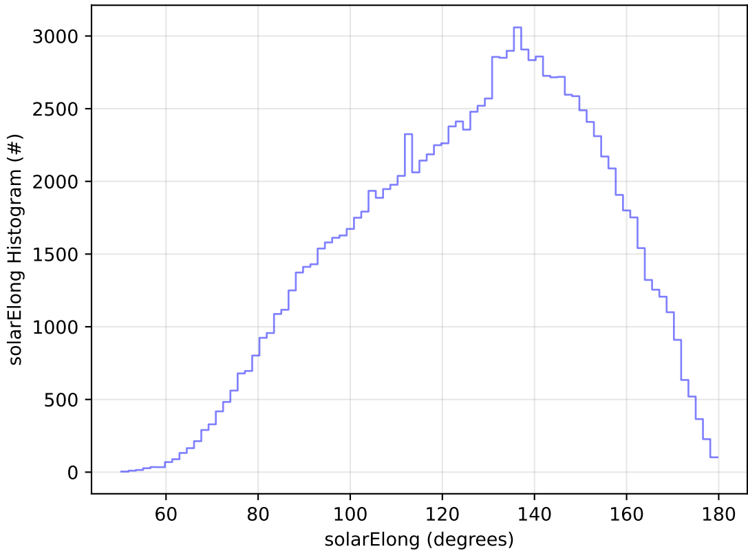
ddf_acor_sf25_lsf40_lsr20_v3.4_10yrs All sky u band: solarElong Histogram
