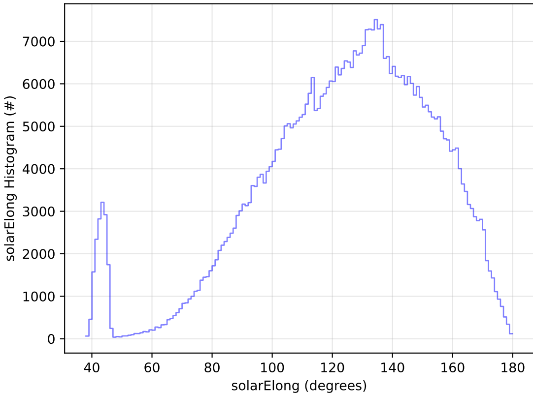
ddf_acor_sf25_lsf40_lsr20_v3.4_10yrs All sky r band: solarElong Histogram
