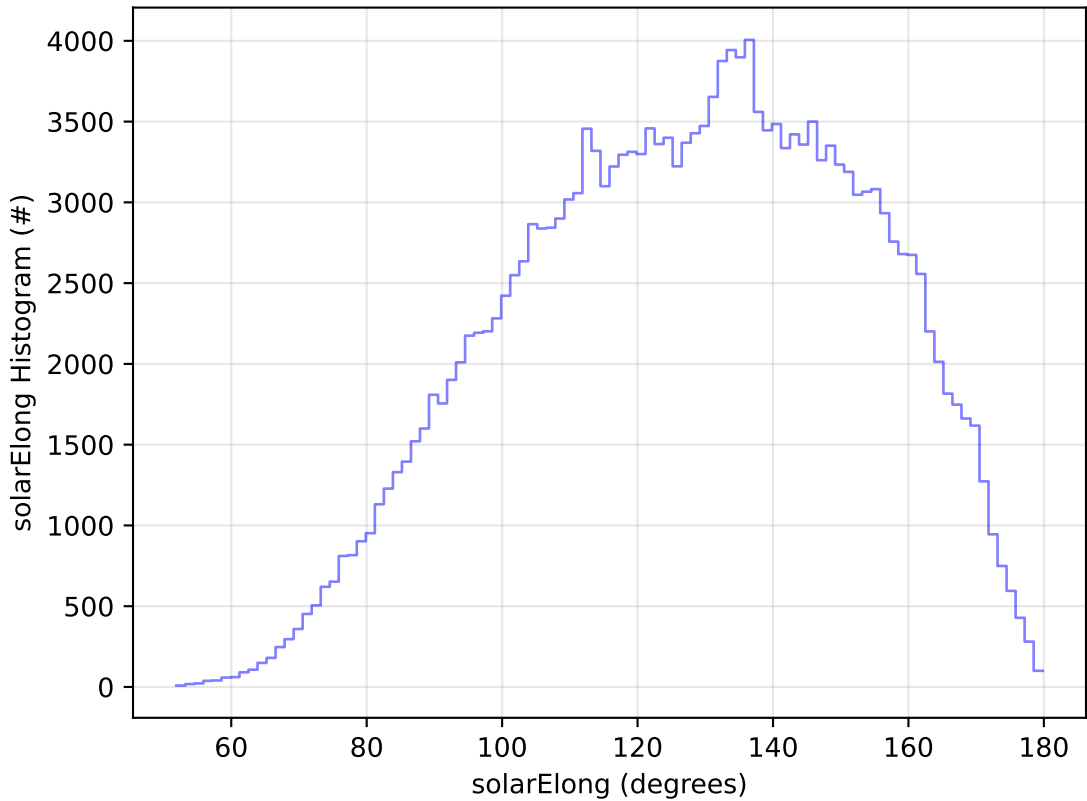
ddf_acor_sf25_lsf40_lsr20_v3.4_10yrs All sky g band: solarElong Histogram
