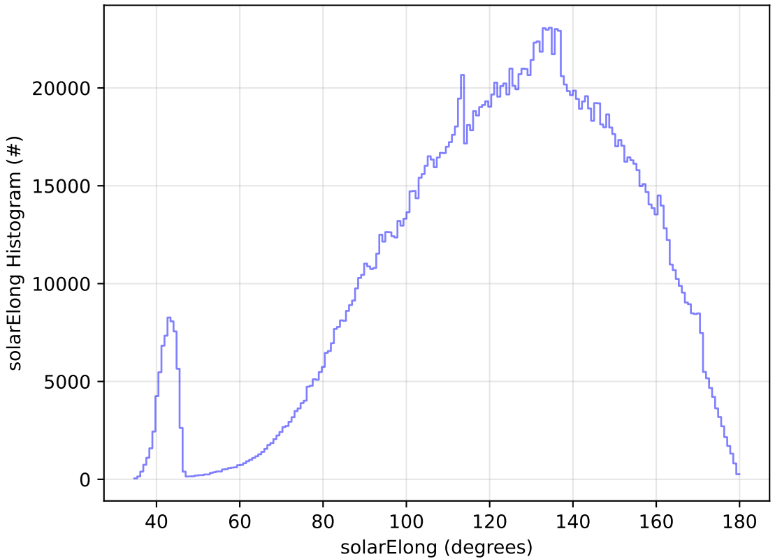
ddf_acor_sf25_lsf40_lsr20_v3.4_10yrs All sky all bands: solarElong Histogram
