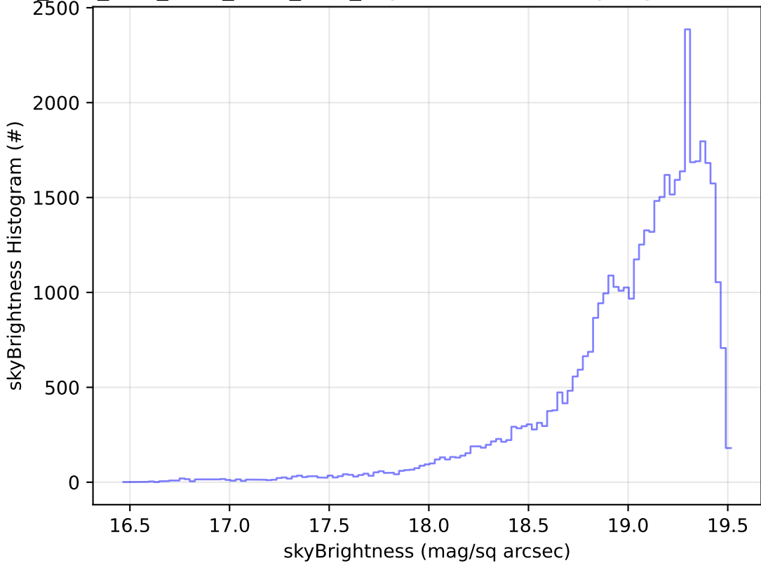
ddf_acor_sf25_lsf40_lsr20_v3.4_10yrs Yr 1 z band: skyBrightness Histogram
