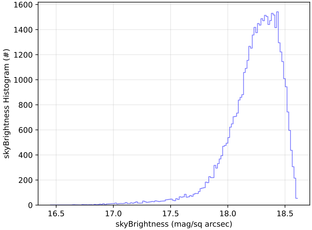
ddf_acor_sf25_lsf40_lsr20_v3.4_10yrs Yr 1 y band: skyBrightness Histogram
