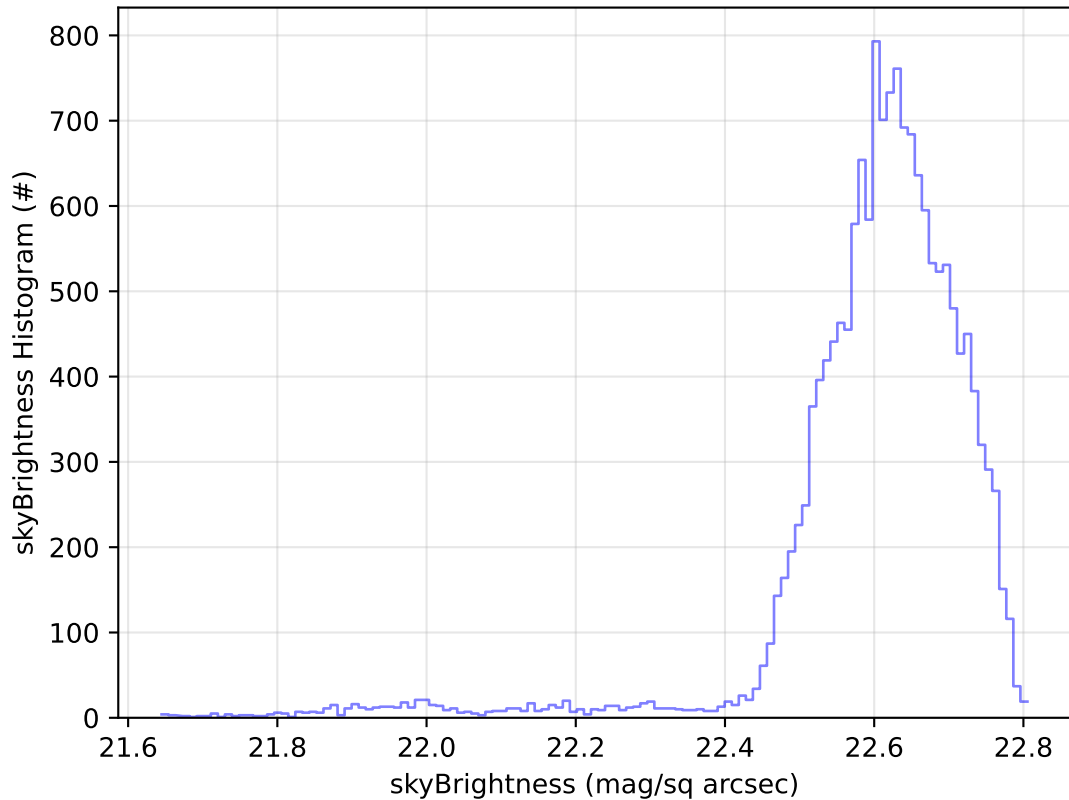
ddf_acor_sf25_lsf40_lsr20_v3.4_10yrs Yr 1 u band: skyBrightness Histogram
