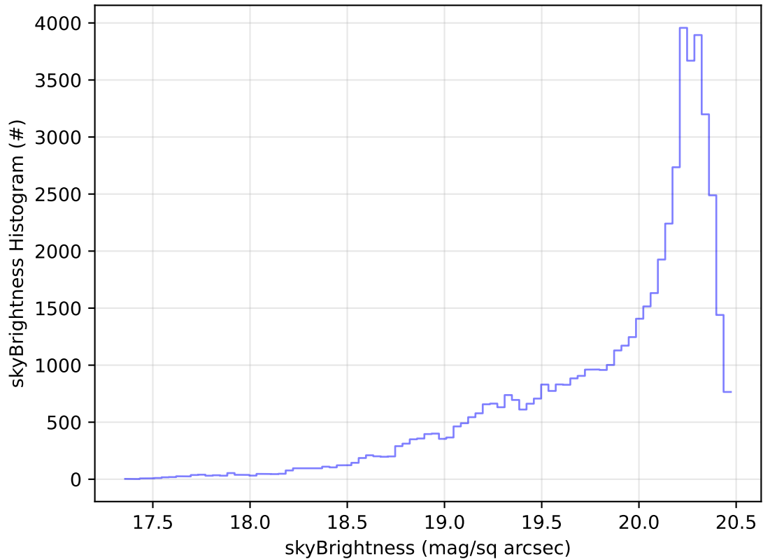
ddf_acor_sf25_lsf40_lsr20_v3.4_10yrs Yr 1 i band: skyBrightness Histogram
