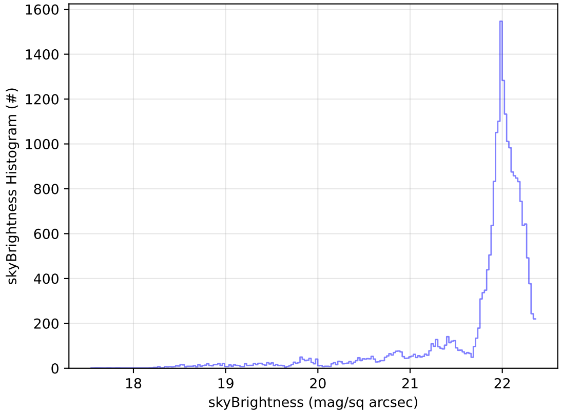
ddf_acor_sf25_lsf40_lsr20_v3.4_10yrs Yr 1 g band: skyBrightness Histogram
