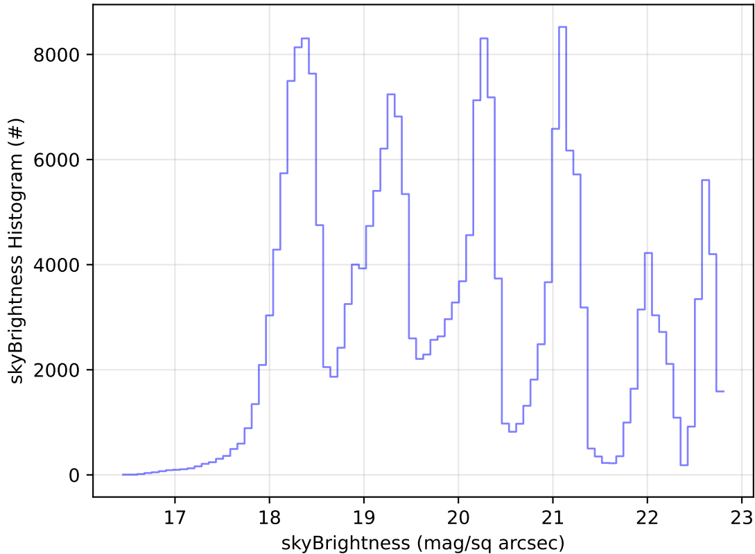
ddf_acor_sf25_lsf40_lsr20_v3.4_10yrs Yr 1 all bands: skyBrightness Histogram
