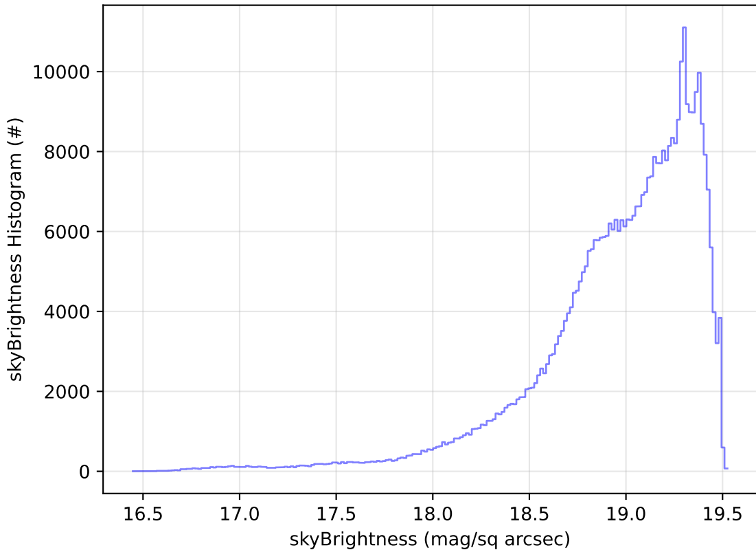
ddf_acor_sf25_lsf40_lsr20_v3.4_10yrs WFD z band: skyBrightness Histogram
