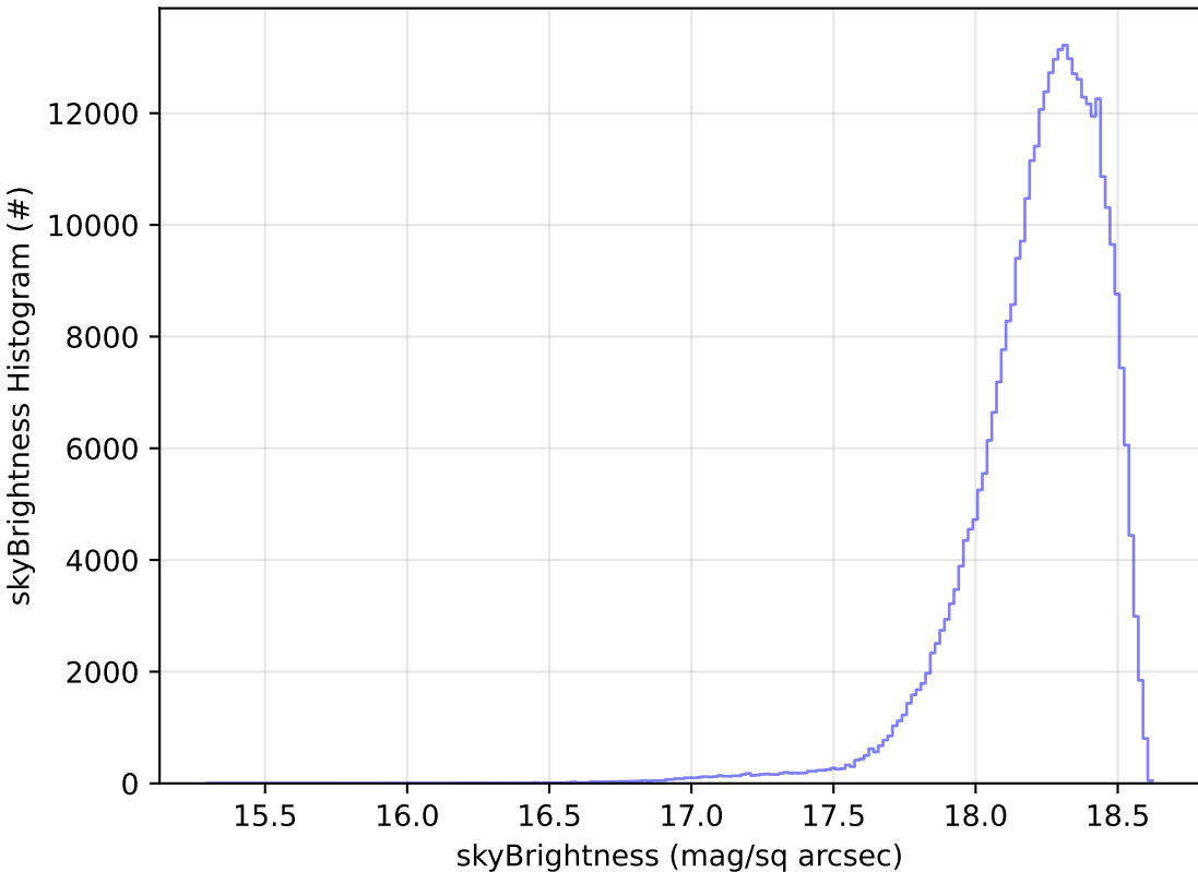
ddf_acor_sf25_lsf40_lsr20_v3.4_10yrs WFD y band: skyBrightness Histogram
