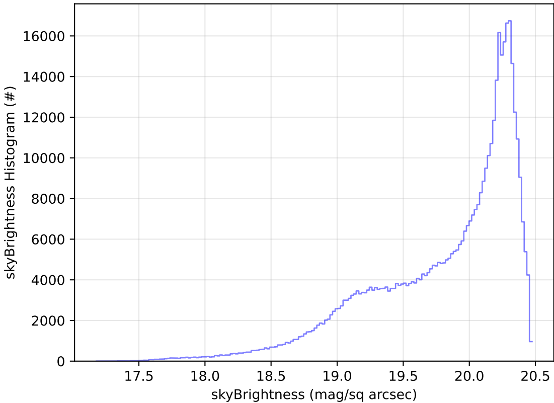
ddf_acor_sf25_lsf40_lsr20_v3.4_10yrs WFD i band: skyBrightness Histogram
