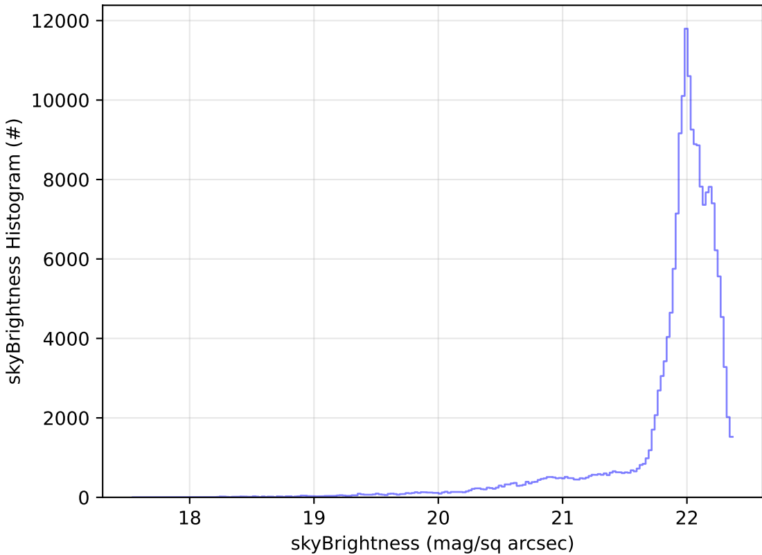
ddf_acor_sf25_lsf40_lsr20_v3.4_10yrs WFD g band: skyBrightness Histogram
