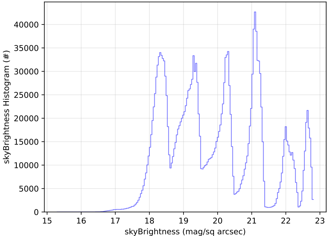
ddf_acor_sf25_lsf40_lsr20_v3.4_10yrs WFD all bands: skyBrightness Histogram
