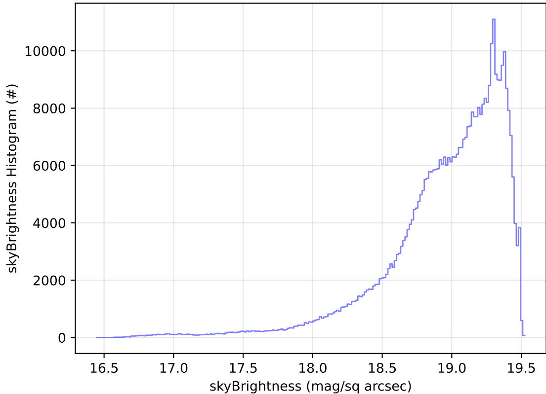
ddf_acor_sf25_lsf40_lsr20_v3.4_10yrs All sky z band: skyBrightness Histogram
