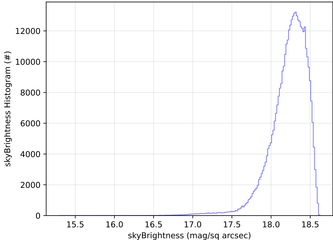
ddf_acor_sf25_lsf40_lsr20_v3.4_10yrs All sky y band: skyBrightness Histogram
