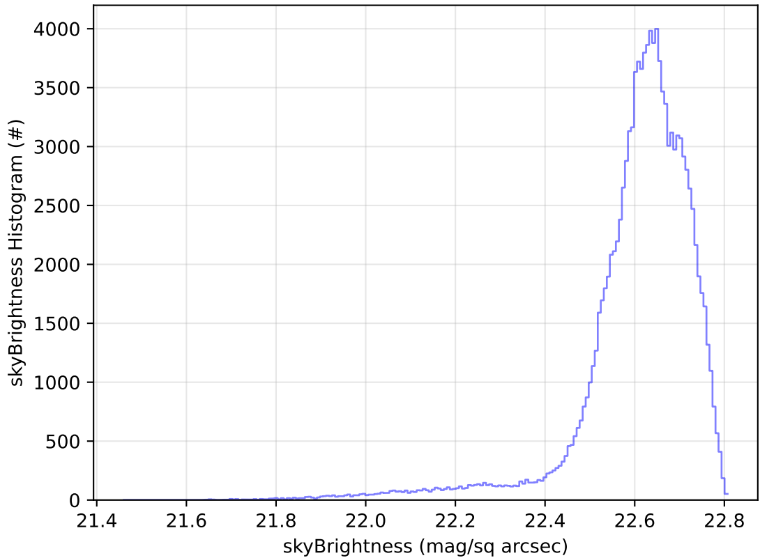
ddf_acor_sf25_lsf40_lsr20_v3.4_10yrs All sky u band: skyBrightness Histogram
