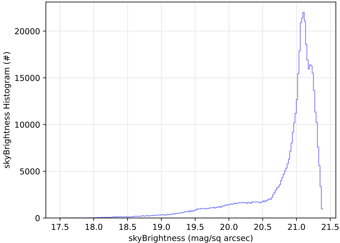
ddf_acor_sf25_lsf40_lsr20_v3.4_10yrs All sky r band: skyBrightness Histogram
