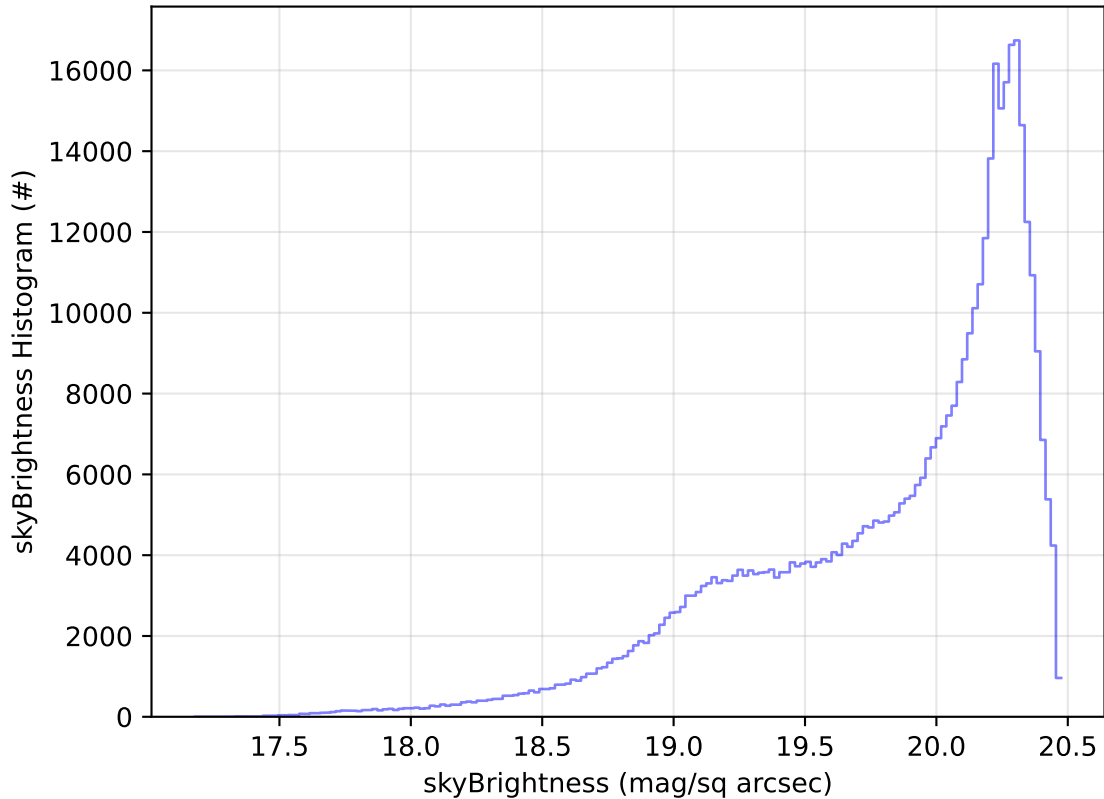
ddf_acor_sf25_lsf40_lsr20_v3.4_10yrs All sky i band: skyBrightness Histogram
