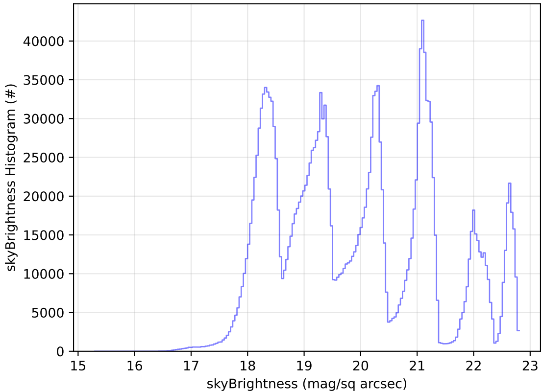
ddf_acor_sf25_lsf40_lsr20_v3.4_10yrs All sky all bands: skyBrightness Histogram
