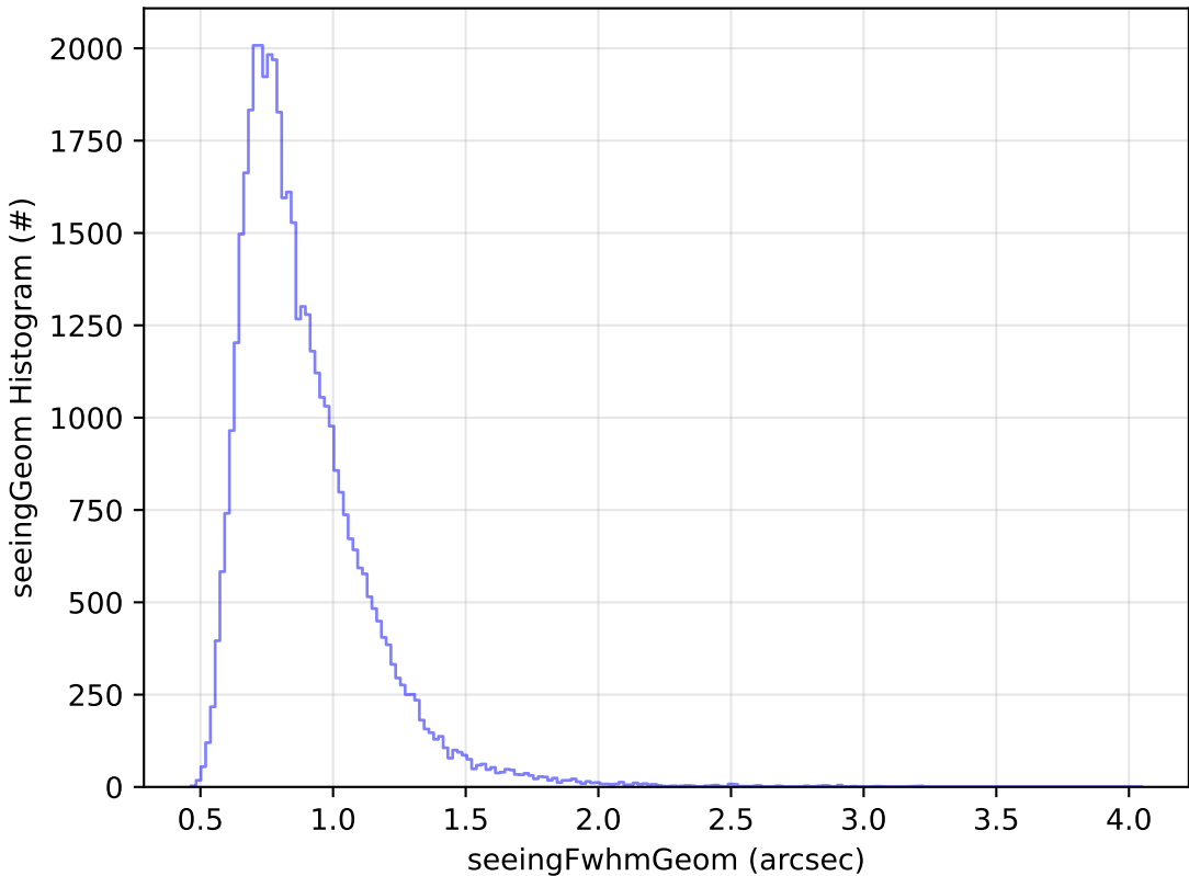
ddf_acor_sf25_lsf40_lsr20_v3.4_10yrs Yr 1 z band: seeingGeom Histogram
