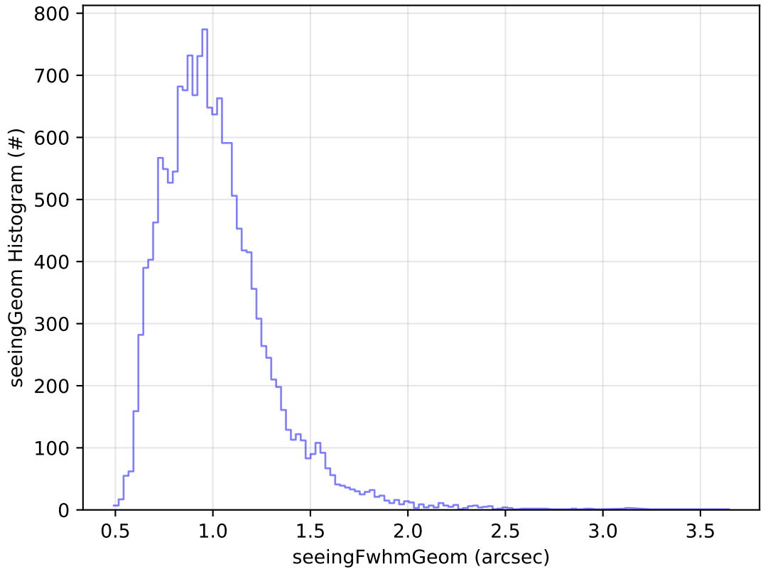
ddf_acor_sf25_Isf40_Isr20_v3.4_10yrs Yr 1 u band: seeingGeom Histogram
