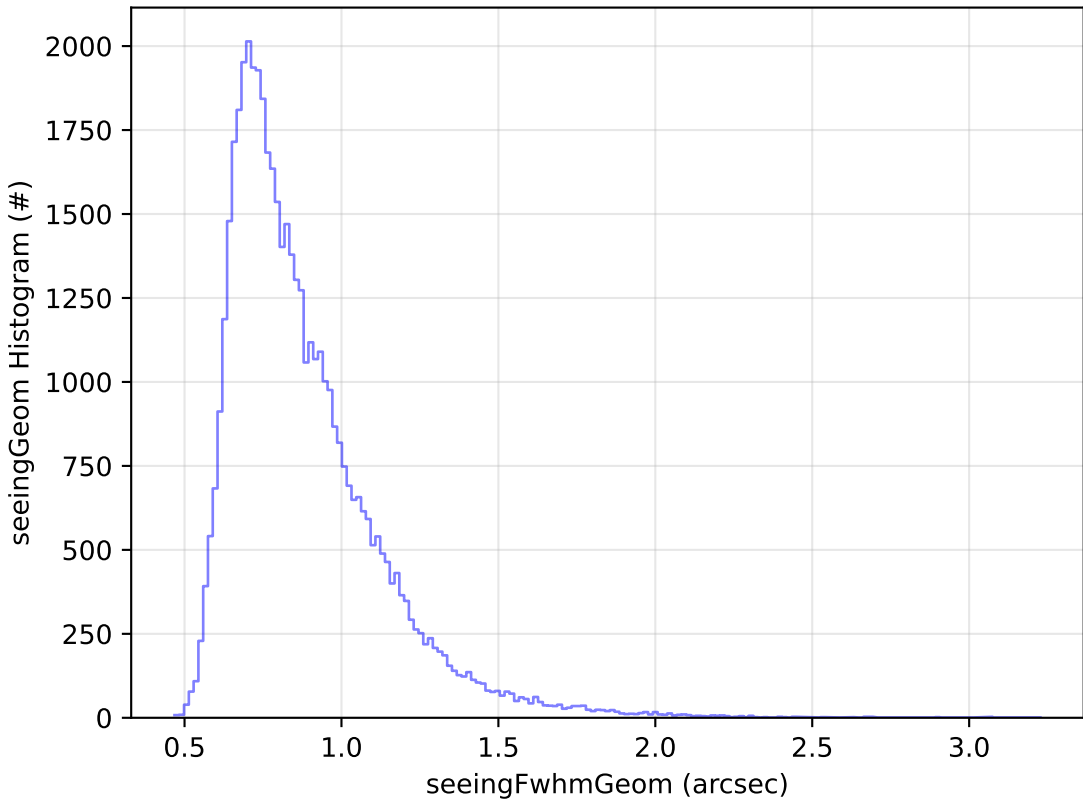
ddf_acor_sf25_lsf40_lsr20_v3.4_10yrs Yr 1 r band: seeingGeom Histogram
