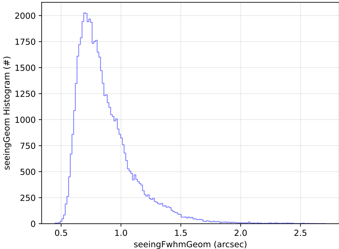
ddf_acor_sf25_lsf40_lsr20_v3.4_10yrs Yr 1 i band: seeingGeom Histogram
