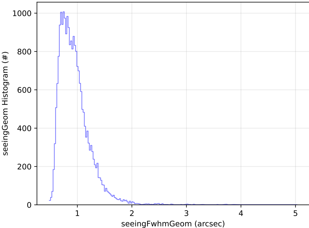
ddf_acor_sf25_lsf40_lsr20_v3.4_10yrs Yr 1 g band: seeingGeom Histogram
