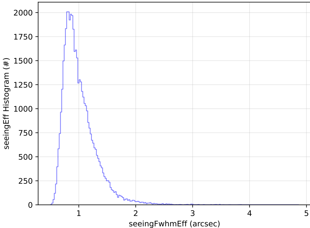
ddf_acor_sf25_lsf40_lsr20_v3.4_10yrs Yr 1 z band: seeingEff Histogram
