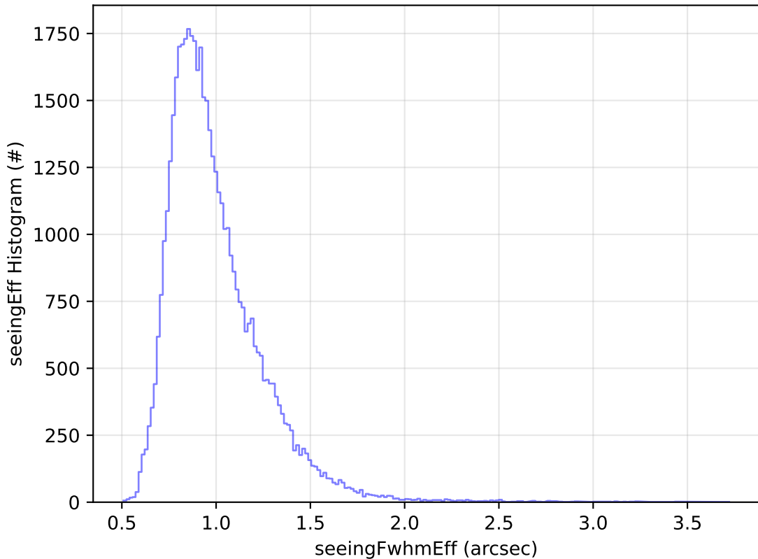
ddf_acor_sf25_lsf40_lsr20_v3.4_10yrs Yr 1 y band: seeingEff Histogram
