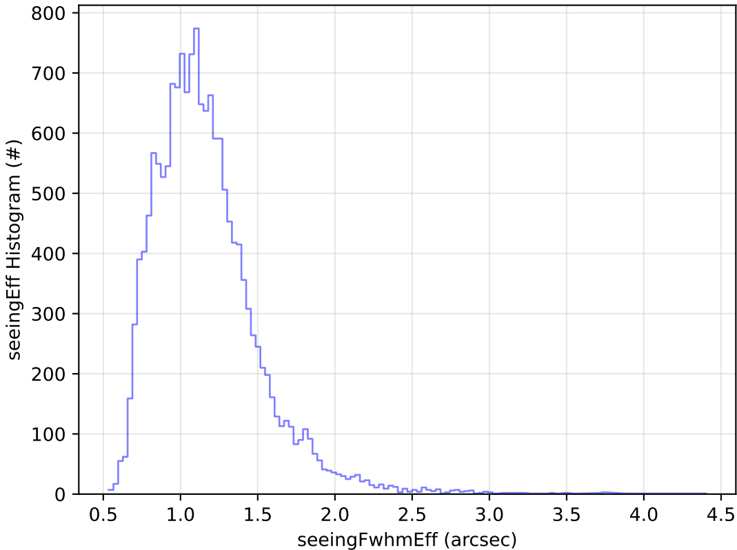
ddf_acor_sf25_lsf40_lsr20_v3.4_10yrs Yr 1 u band: seeingEff Histogram
