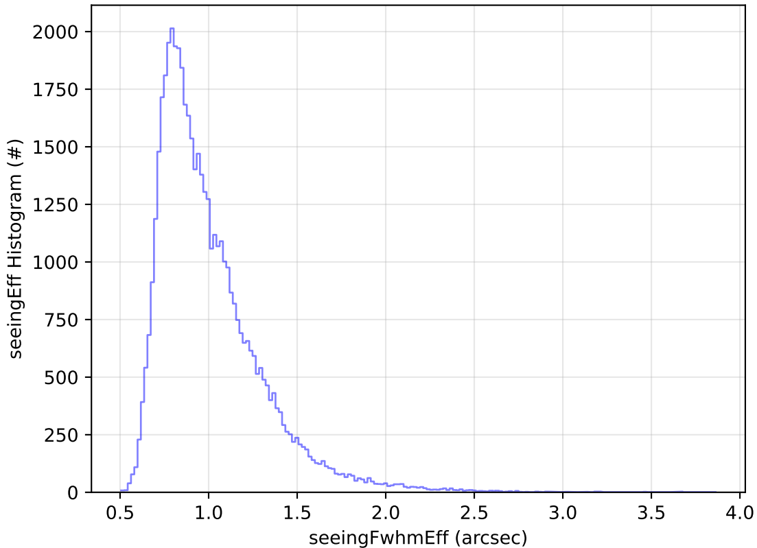
ddf_acor_sf25_lsf40_lsr20_v3.4_10yrs Yr 1 r band: seeingEff Histogram
