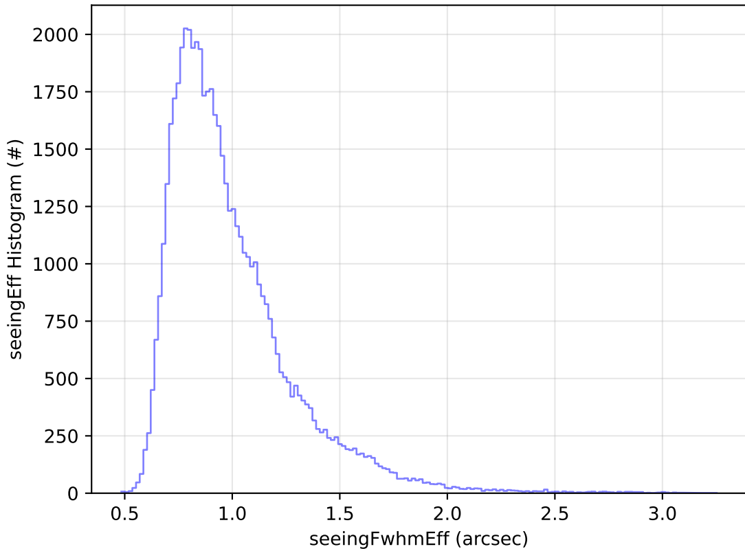
ddf_acor_sf25_lsf40_lsr20_v3.4_10yrs Yr 1 i band: seeingEff Histogram
