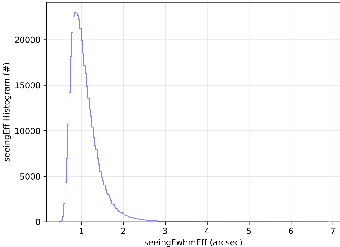
ddf_acor_sf25_lsf40_lsr20_v3.4_10yrs WFD z band: seeingEff Histogram
