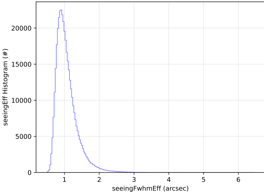
ddf_acor_sf25_lsf40_lsr20_v3.4_10yrs WFD y band: seeingEff Histogram
