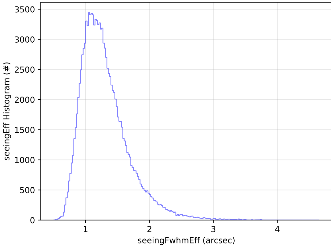
ddf_acor_sf25_lsf40_lsr20_v3.4_10yrs WFD u band: seeingEff Histogram
