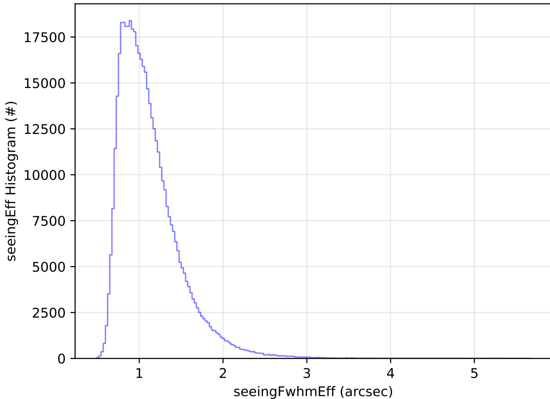
ddf_acor_sf25_lsf40_lsr20_v3.4_10yrs WFD r band: seeingEff Histogram
