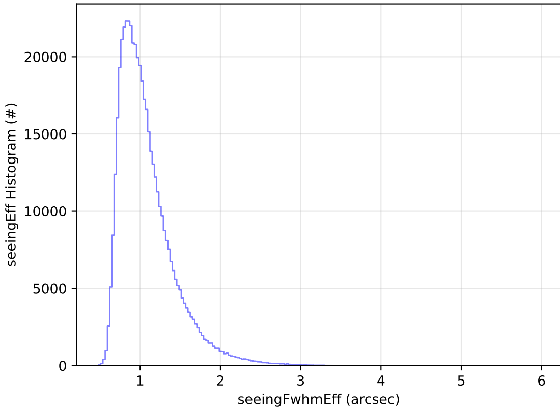
ddf_acor_sf25_lsf40_lsr20_v3.4_10yrs WFD i band: seeingEff Histogram
