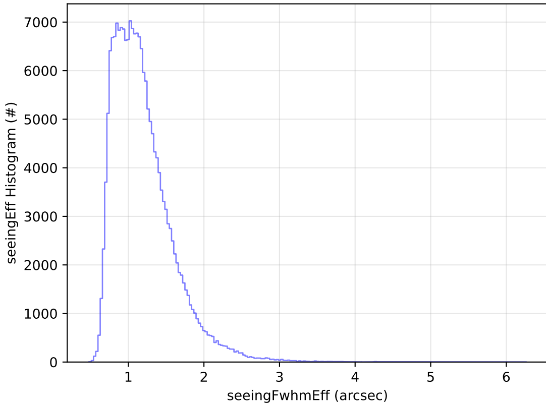
ddf_acor_sf25_lsf40_lsr20_v3.4_10yrs WFD g band: seeingEff Histogram
