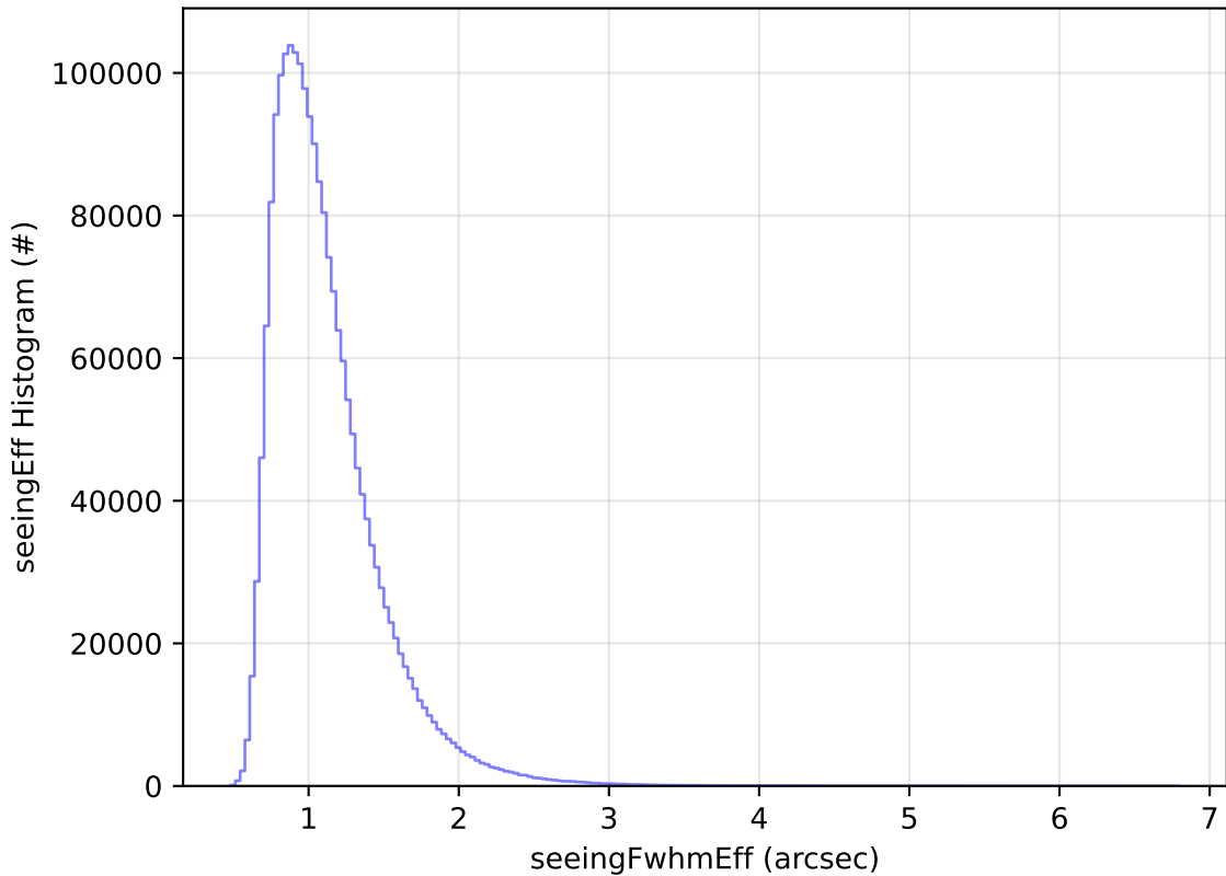
ddf_acor_sf25_lsf40_lsr20_v3.4_10yrs WFD all bands: seeingEff Histogram
