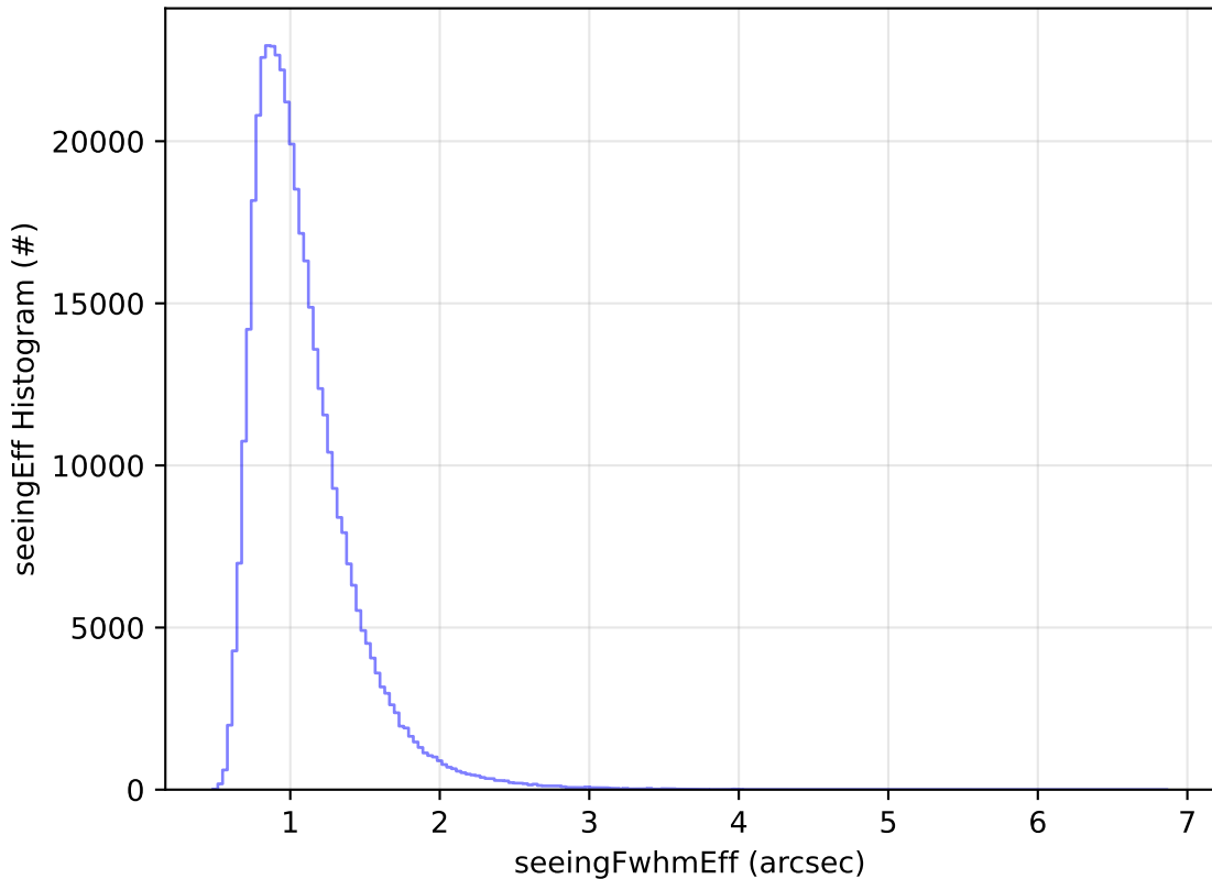
ddf_acor_sf25_Isf40_Isr20_v3.4_10yrs All sky z band: seeingEff Histogram
