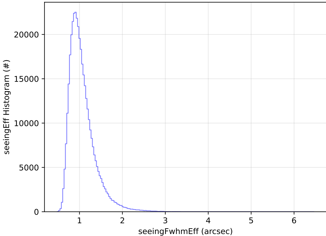
ddf_acor_sf25_lsf40_lsr20_v3.4_10yrs All sky y band: seeingEff Histogram
