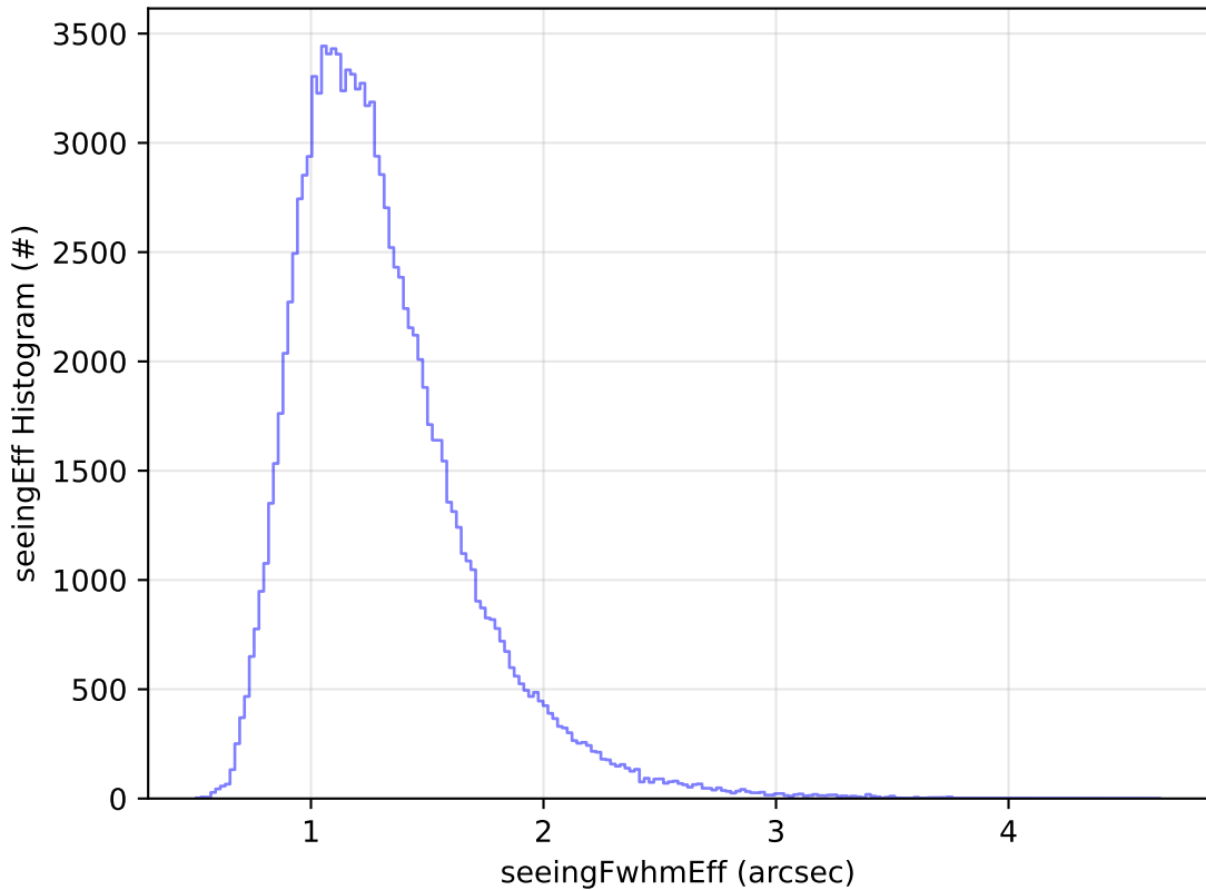
ddf_acor_sf25_ls40_lsr20_v3.4_10yrs All sky u band: seeingEff Histogram
