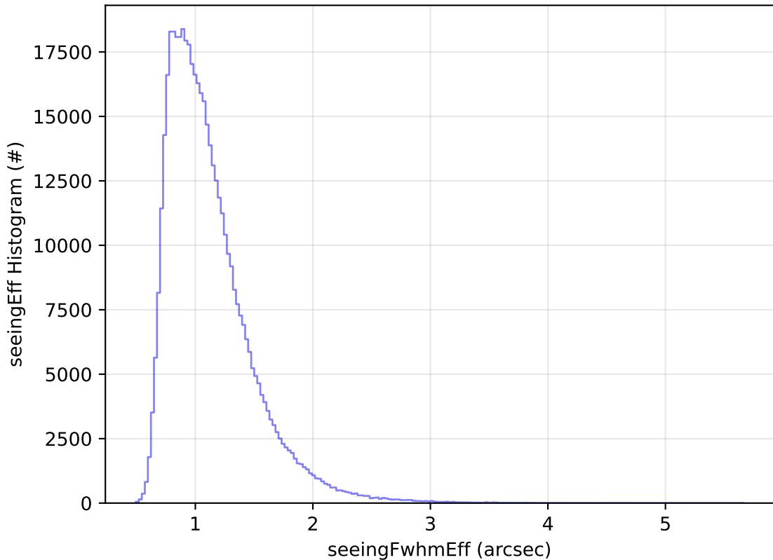
ddf_acor_sf25_lsf40_lsr20_v3.4_10yrs All sky r band: seeingEff Histogram
