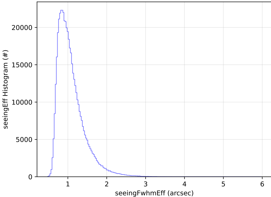
ddf_acor_sf25_lsf40_lsr20_v3.4_10yrs All sky i band: seeingEff Histogram
