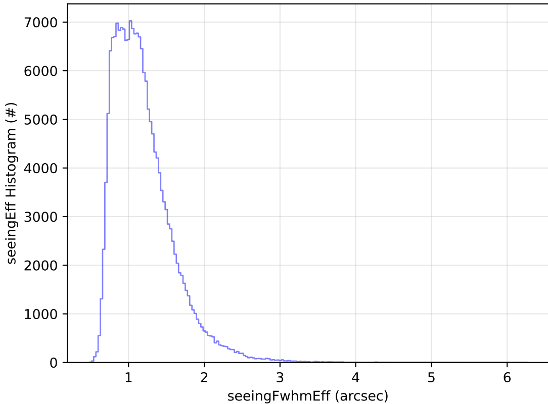
ddf_acor_sf25_ls40_lsr20_v3.4_10yrs All sky g band: seeingEff Histogram
