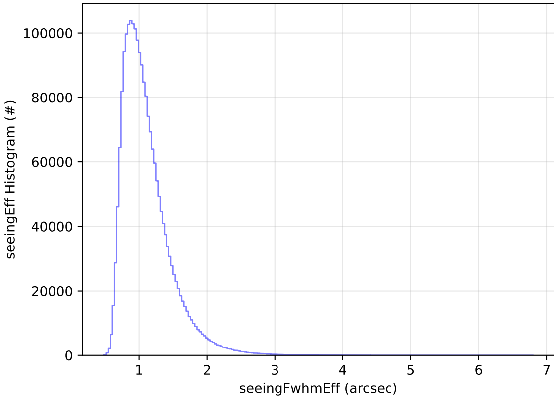
ddf_acor_sf25_lsf40_lsr20_v3.4_10yrs All sky all bands: seeingEff Histogram
