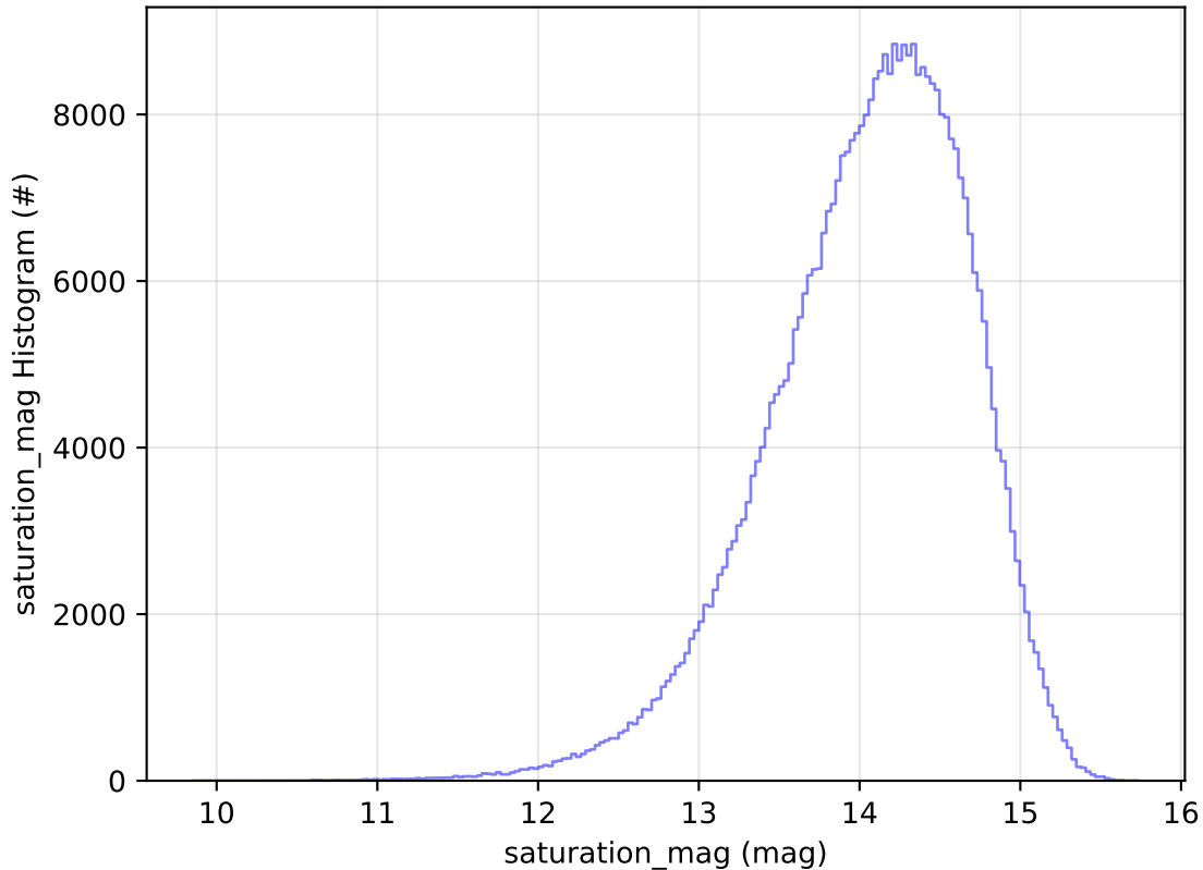
ddf_acor_sf25_lsf40_lsr20_v3.4_10yrs WFD z band: saturation_mag Histogram
