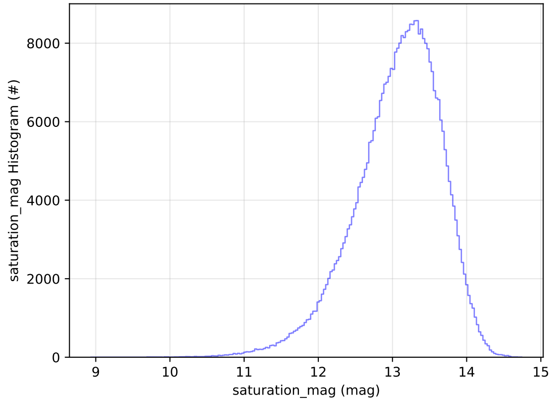
ddf_acor_sf25_lsf40_lsr20_v3.4_10yrs WFD y band: saturation_mag Histogram
