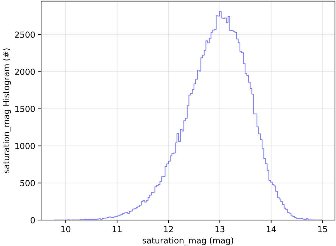
ddf_acor_sf25_lsf40_lsr20_v3.4_10yrs WFD u band: saturation_mag Histogram
